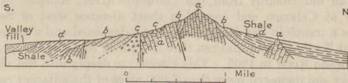
FIGURE 70.—Section across Coyote Mountain, Calif., near Alverson and Garnett Canyons. After Mendenhall. a , Limestone (Paleozoic) metamorphosed to marble by intrusive granite; b , sandstone and conglomerate; c , tuff (Miocene); d , shale (Miocene)
