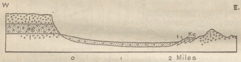
FIGURE 14.—Section across the Alpine Basin just north of Alpine, Tex. I, Lava (Tertiary); ag, agglomerate; Kc, limestone (Comanche).
