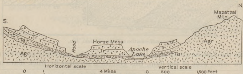
FIGURE 58.—Section showing relations of Tertiary volcanic succession 15 miles southwest of Roosevelt Dam, Ariz. Tr, Rhyolite tuff; Ta, andesite; Agr, granite
