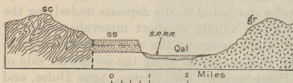
FIGURE 64.—Cross section of San Gorgonio Pass near Cabazon siding, Calif., looking east. gr, granite; ss, sandstone; sc, schist; Qal, alluvium
