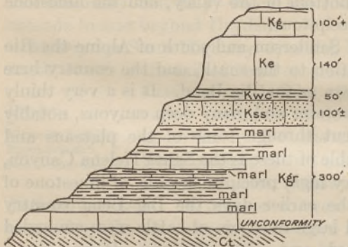
FIGURE 9.—Section near Maxon, Tex. Cretaceous: K&g, Georgetown limestone; Ke, Edwards limestone; Kwc, Walnut and Comanche Peak limestones; Kss, sandstone; K&g, Glen Rose formation. Pennsylvanian: Ct, Tesnus formation
