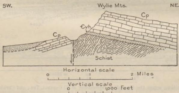
FIGURE 21.—Section across the western part of the Wylie Mountains north of Lobo siding, Tex. Cp, Permian limestone; Evh, Van Horn sandstone (Cambrian)
