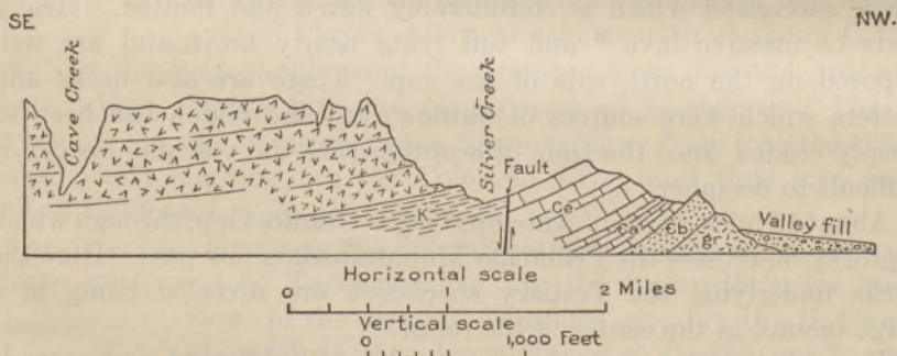
FIGURE 43.—Section of northeastern foothills of Chiricahua Mountains near Portal, Ariz. Cb, quartzite with sills of rhyolite (Cambrian); Ca, thin-bedded limestone and shale (Abrigo); Ce, limestone (Devonian and Carboniferous); K, sandstone, limestone, and shale (Comanche, Lower Cretaceous); Tv, lava (latite, Tertiary), dipping south at a low angle; gr, granite
