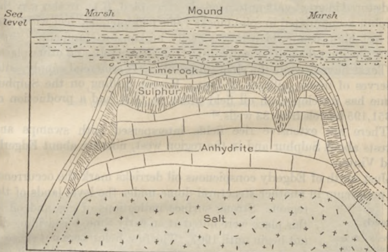
FIGURE 2.—Section across dome near Sulphur, La. After Kelly
