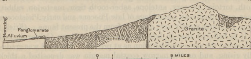
FIGURE 65.—Section from Banning, Calif., north to San Bernardino Mountain. After Vaughan
