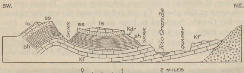
FIGURE 27.—Section southwest from cement quarry 2 miles west of El Paso, Tex. Is, Limestone, and ss, sandstone, of Upper Cretaceous age; Kdr, Del Rio horizon; sh, dark shale; Kf, Fredericksburg group; Tp, intrusive porphyry
