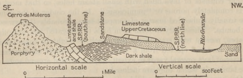
FIGURE 40.—Section through Bowen siding, New Mexico
