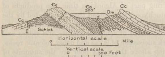
FIGURE 48.—Section at Picacho de la Calera, 16 miles northwest of Tucson, Ariz. Cq, Cambrian quartzite; Ca, Abrigo limestone; Dm, Martin limestone; Cc, Carboniferous limestone; d, dike
