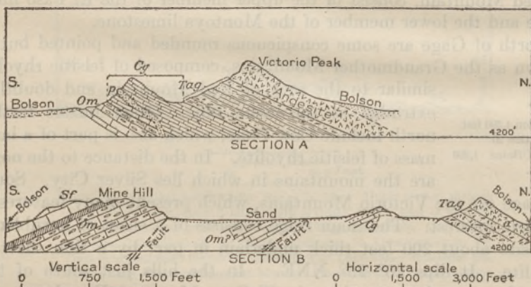
FIGURE 34.—Sections across Victorio Mountains, south of Gage, Luna County, N. Mex. a , Andesite; Tag , agglomerate, shale, and sandstone; Cg , Gym limestone (Permian); Sf , Fusselman limestone; Om , Montoya limestone; p , porphyry dike
