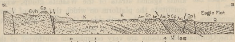
FIGURE 22.—Section from the southern edge of the Diablo Plateau to Eagle Flat, east of the Sierra Blanca, Tex. By P. B. King. K, Sandstone and limestone (Cretaceous); Cp, limestone (Permian); Evh, Van Horn sandstone (Cambrian); Am, Millican formation (Algonkian), including breccia (br) and diabase (b); Ac, Carrizo Mountain schist; Q, Quaternary sand and gravel
