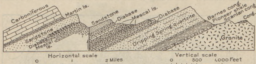
FIGURE 52.—Section across the center of Hayes Mountain, southwest of San Carlos, Ariz.
