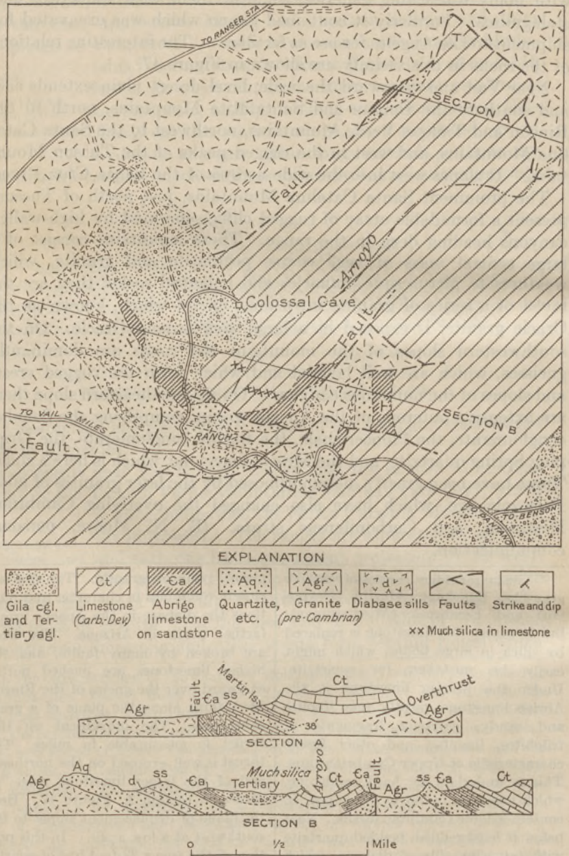
FIGURE 47.—Geologic map and cross sections in the vicinity of Colossal Cave, 3 miles east of Vail, Ariz.
