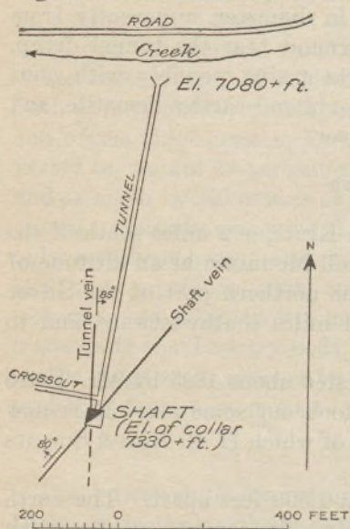
FIGURE 6.—Diagram showing relations of veins and workings in the Silkworm mine.
