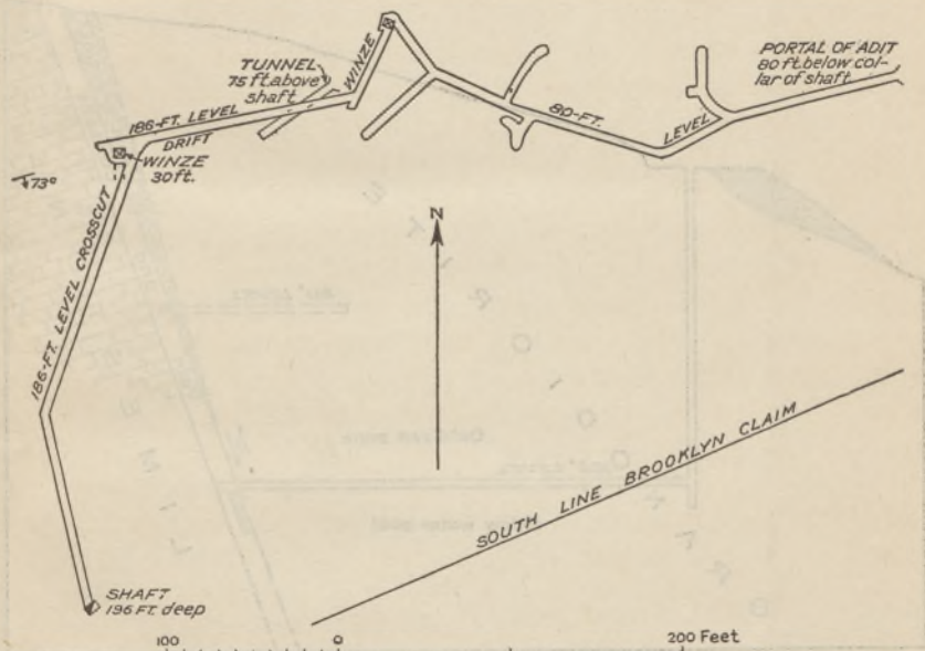
FIGURE 2.—Diagrammatic sketch of Brooklyn workings. From map furnished by the Brooklyn Mining Co.
