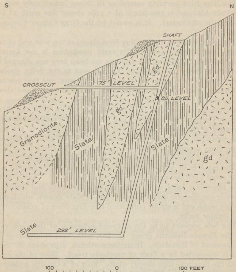
FIGURE 5.—Geologic cross section through the Palo Alto shaft. After J. T. Bailey, Eng. and Min. Jour., vol. 76, p. 613, 1903.
