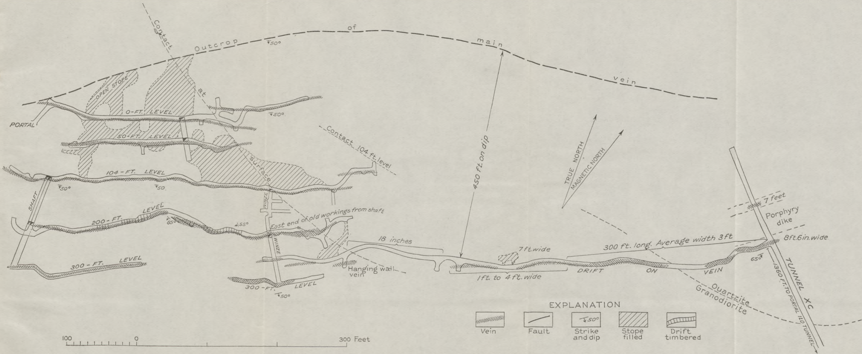
GEOLOGIC SKETCH MAP OF THE NEVADA-BELLEVUE MINE.
