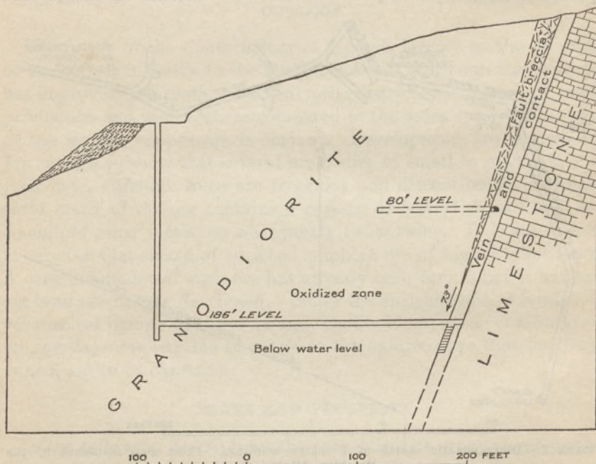
FIGURE 3.—Diagrammatic geologic section through the Brooklyn mine.
