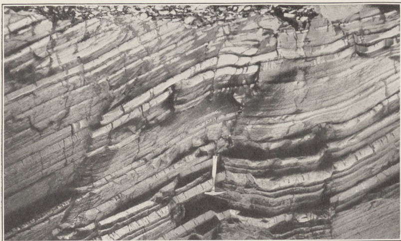
B. INTERBEDDED SLATE AND GRAYWACKE, IZHUT BAY, AFOGNAK ISLAND.
