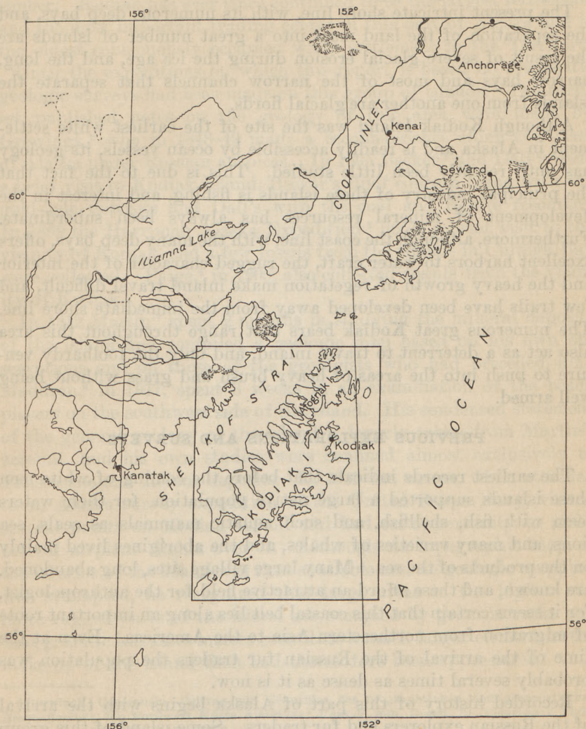
FIGURE 5.—Index map showing location of Kodiak and adjacent islands. The area shown on plate 2 is indicated by the rectangle enclosing Kodiak and the adjacent islands.
