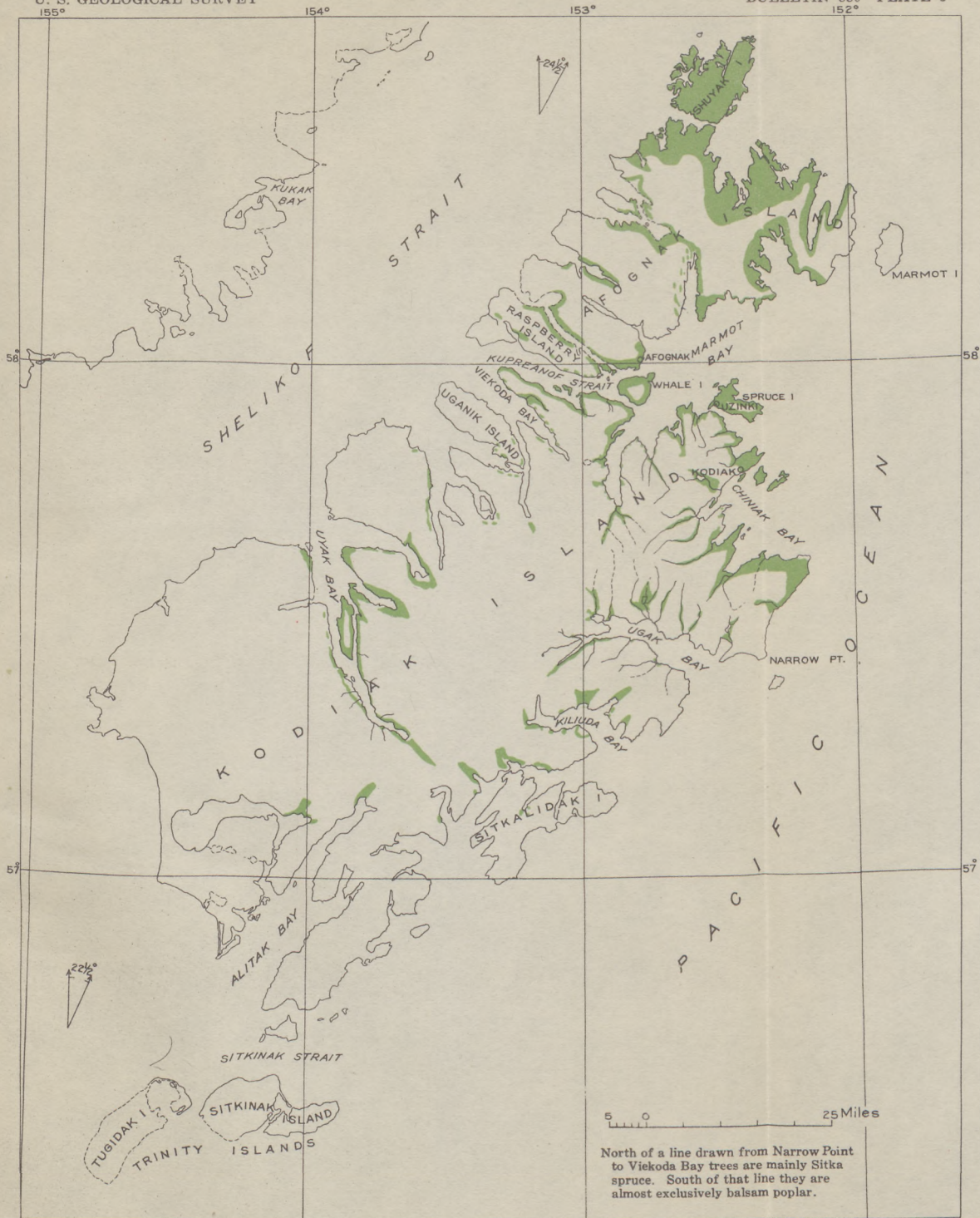
MAP OF KODIAK AND ADJACENT ISLANDS SHOWING AREAS IN WHICH TREES OCCUR
