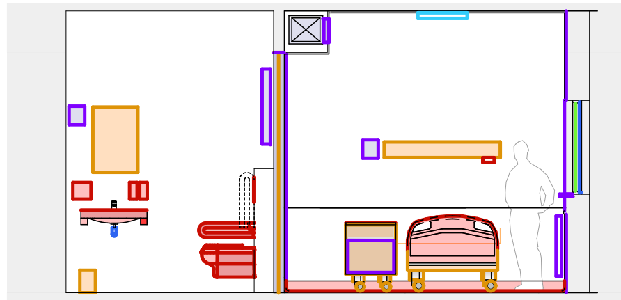
A plan of a patient room with an en-suite bathroom
