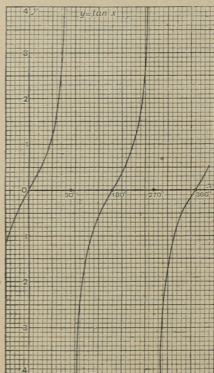
y = \tan x.
