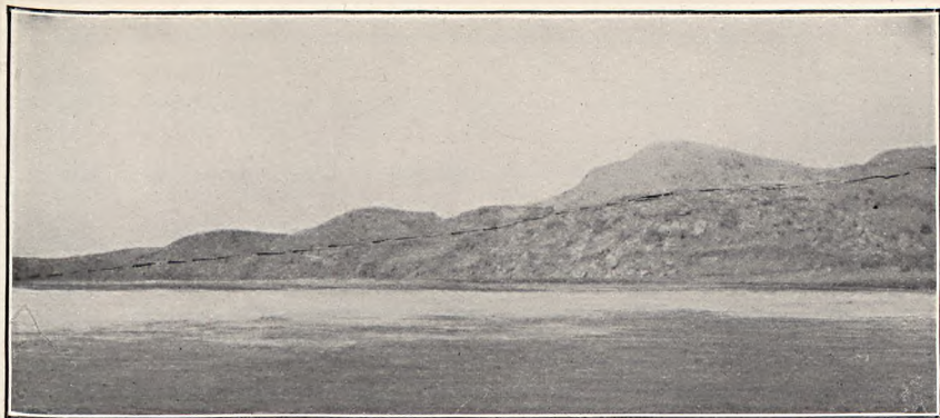
A. NORTH BLUFF OF RED RIVER IN NE. \frac{1}{4} SEC. 31, T. 5 S., R. 12 W. Showing westward dip of Permian rocks.
