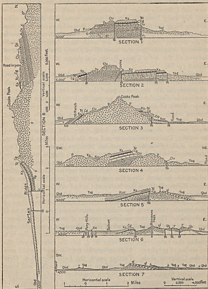
FIGURE 3.—Sections across Cooks Range. 1, 1\frac{1}{2} miles north of Cooks post office; 2, through Cooks post office; 3, through Cooks Peak; 4, 2 to 3 miles south of Cooks Peak; 5, 1\frac{1}{2} miles north of Fort Cummings; 6, 1\frac{1}{2} miles south of Fort Cummings, passing just south of sandstone quarry; 7, from point 1\frac{1}{2} miles southeast of Fluorite Camp to point 1\frac{1}{2} miles northwest of Florida station; 8, through Cooks Range from southeast end of Sarten Ridge to the Luna-Sierra county line. Base of sections 1-4, 5,000 feet above sea level; 6-8, 4,500 feet. p, Porphyry; Tag, agglomerate; r, rhyolite, andesite, and latite; Qbd, bolson deposits; Kco, Colorado shale; Ks, Sarten sandstone; Fl, Lobo formation; Cg, Gym limestone and Magdalena formation; Clv, Lake Valley limestone; Dp, Percha shale; Sof, Fusselman and Montoya limestones; Oe, El Paso limestone; E, Bliss sandstone; gr, granite; a, andesite; Qb, quartz basalt; ql, quartz latite; k, keratophyre.
