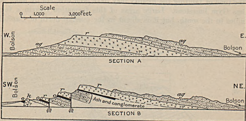
FIGURE 7.—Sections across the Little Florida Mountains. A, Across center of range; B, 1\frac{1}{4} miles farther south. ag , Agglomerate; r , felsitic rhyolite; o , obsidian; k , keratophyre.
