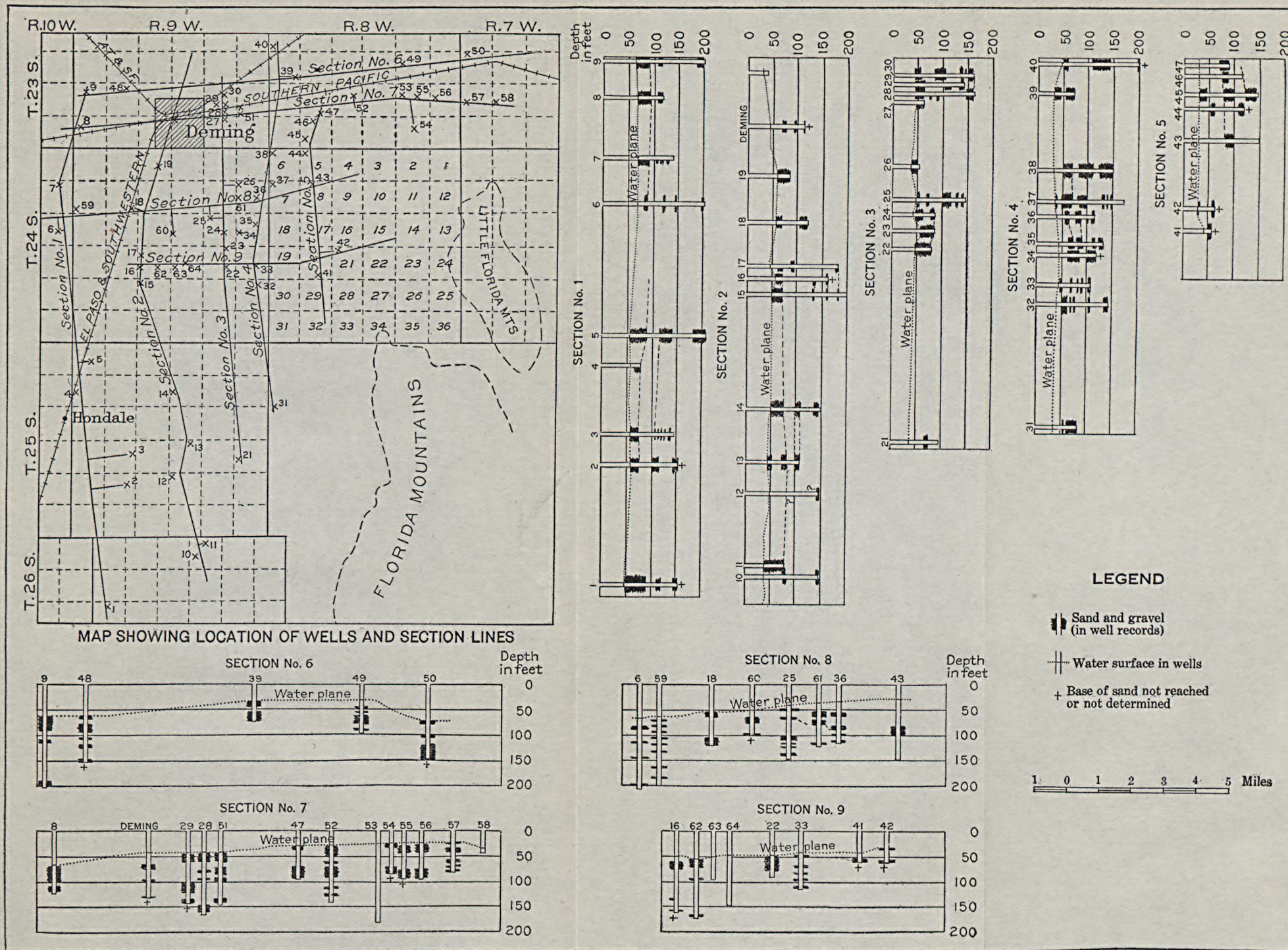
MAP AND SECTIONS SHOWING RELATIONS OF THE WATER-BEARING STRATA IN THE DEMING REGION.
