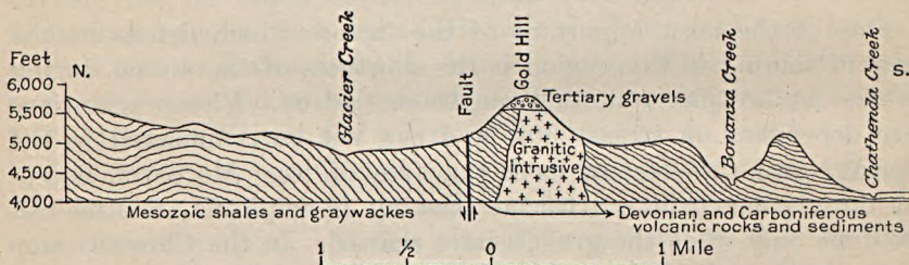
FIGURE 8.—Diagrammatic section through Gold Hill, to show relations of Tertiary gravels to the older formations.
