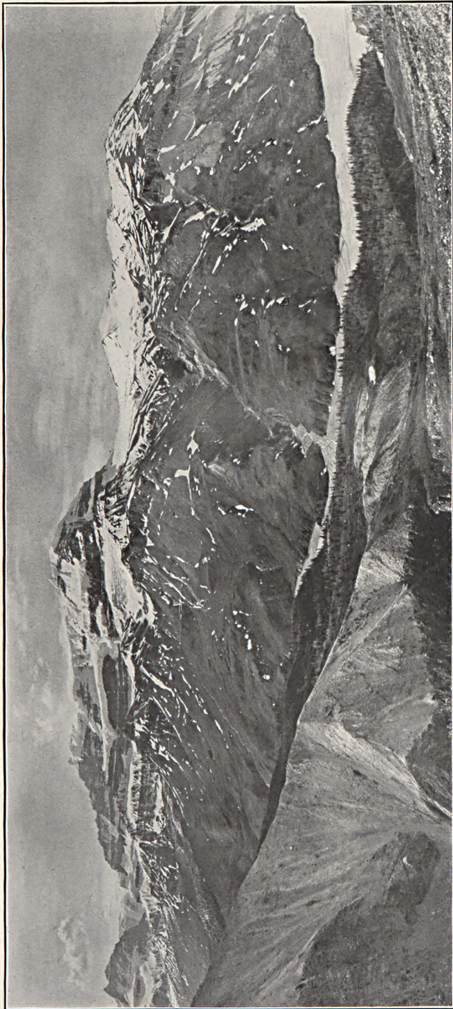
CARBONIFEROUS LAVAS AND SEDIMENTS overlain by younger volcanic rocks on lower Skolai Creek.
