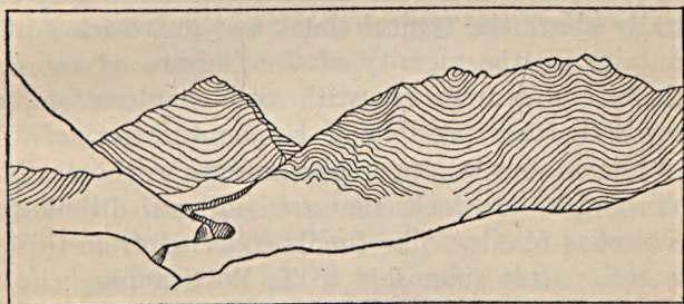
FIGURE 5.—Sketch showing structure of Mesozoic argillites and graywackes on upper Chavolda Creek.
