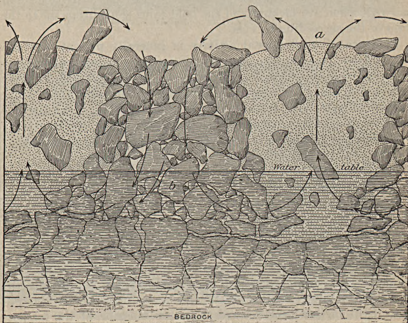
FIGURE 2.—Diagram illustrating segregation of coarse and fine detritus and development of frost-heaved mounds by solifluction.
