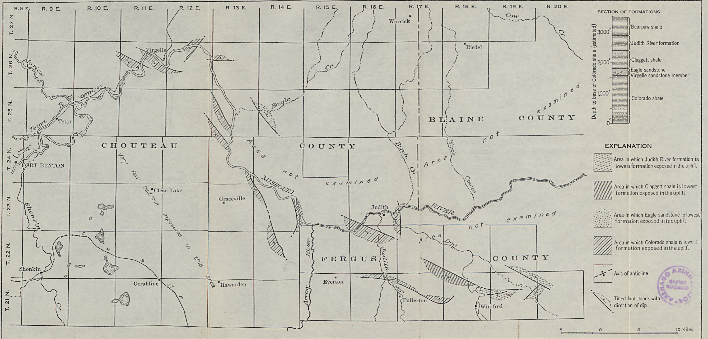
SKETCH MAP SHOWING TILTED AND FOLDED STRUCTURES SOUTH OF THE BEARPAW MOUNTAINS, MONT.
