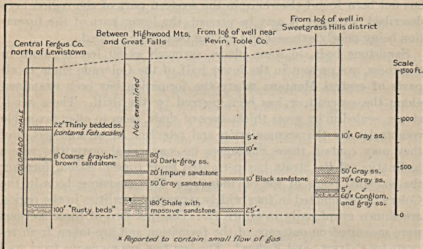
FIGURE 12.—Sections showing sandstones in lower half of Colorado shale, north-central Montana.
