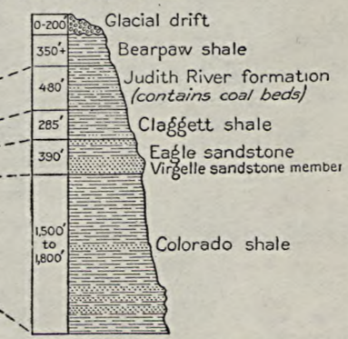
GENERALIZED SECTION OF ROCKS IN THE HAVRE REGION
