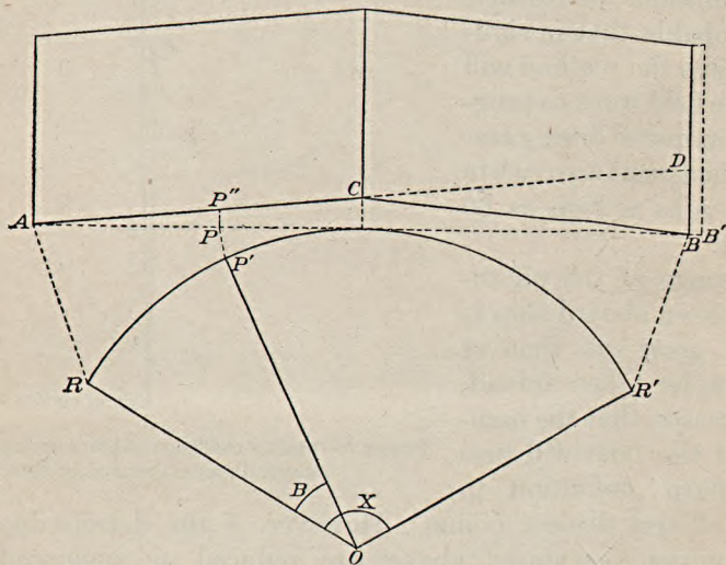
FIGURE 6.—Principles of the panoramic photo-alidade.
