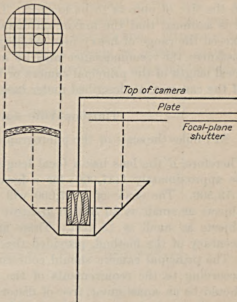
FIGURE 10.—Arrangement of universal level on camera. (After Capt. Ulyanine.)
