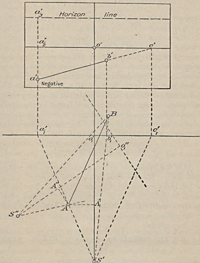
FIGURE 21.—Relative positions of photographic stations. (From Saconney's Métrophotographie .)
