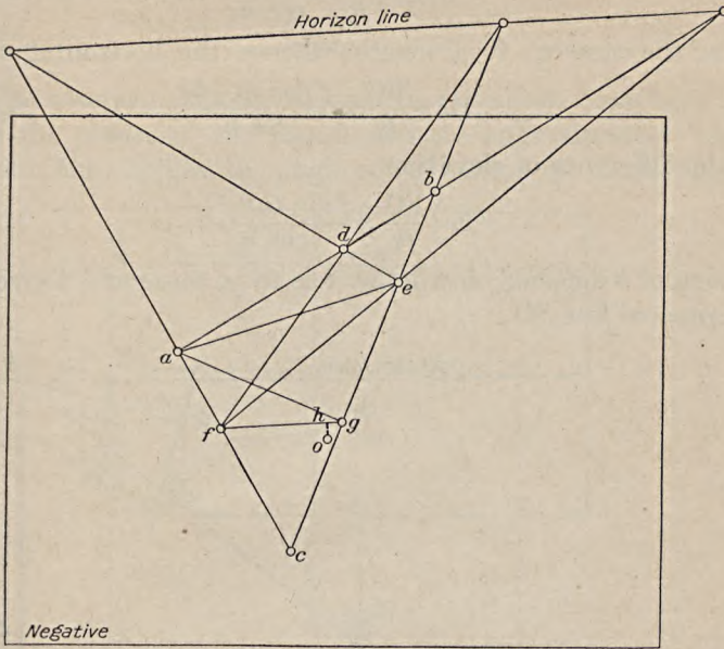
FIGURE 18.—Determination of negative line to locate position of aerial station. (From Saconney's Métrophotographie .)
