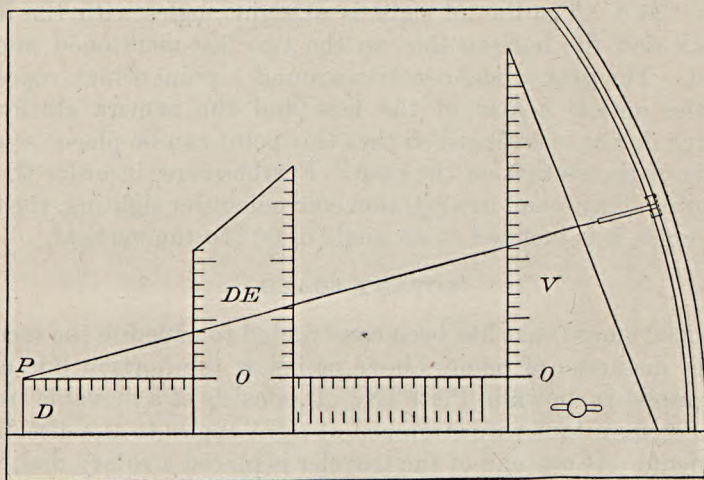
FIGURE 7.—Elevation computer.
