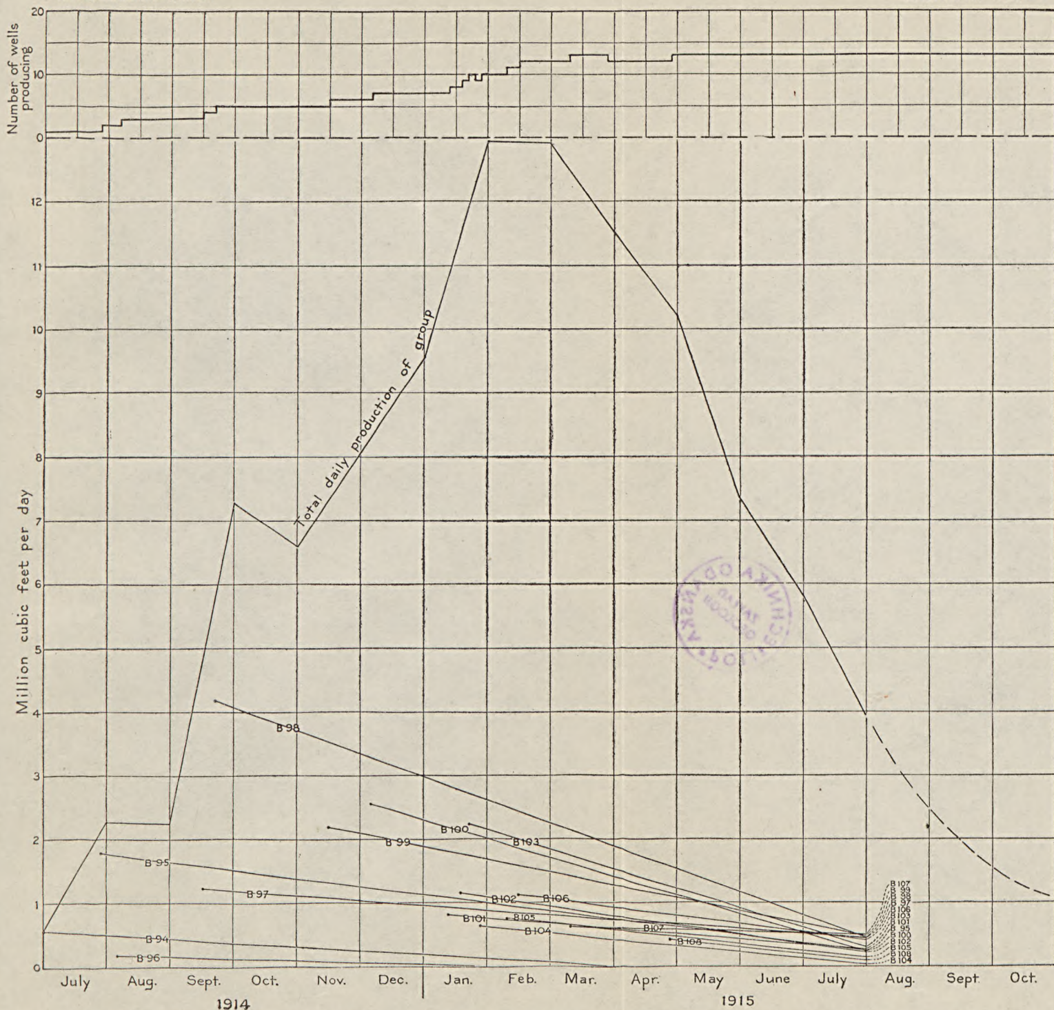
DIAGRAM SHOWING DECLINE IN DAILY PRODUCTION OF 15 WELLS IN WEST PARK GROUP, CLEVELAND, OHIO.
