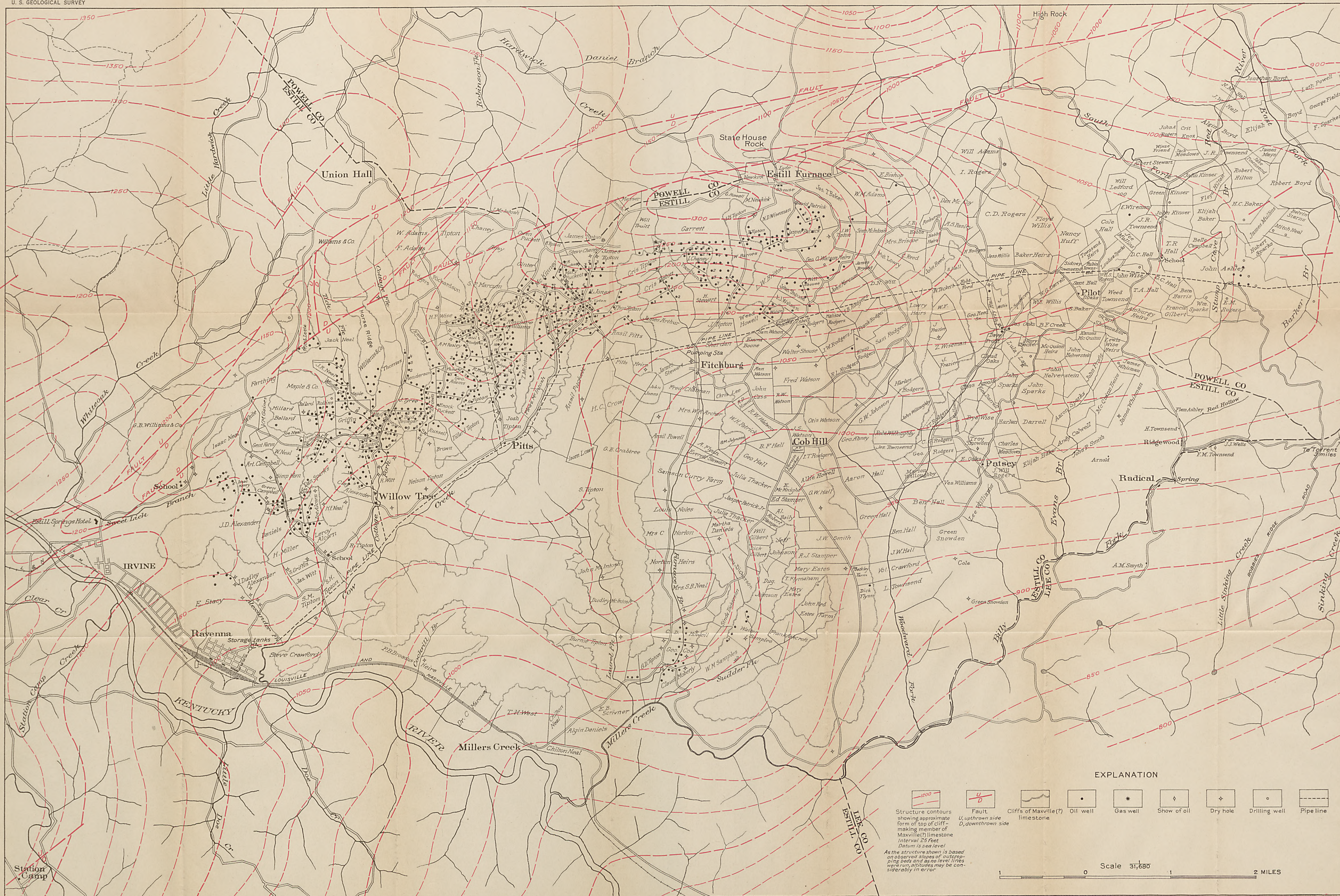
SKETCH MAP OF IRVINE OIL FIELD, KY., SHOWING MAIN FEATURES OF GEOLOGIC STRUCTURE, OIL AND GAS WELLS, AND FARMS
