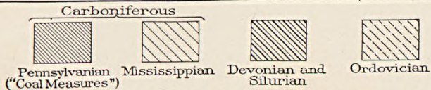
GEOLOGIC SKETCH MAP OF A PART OF NORTHEASTERN KENTUCKY.
