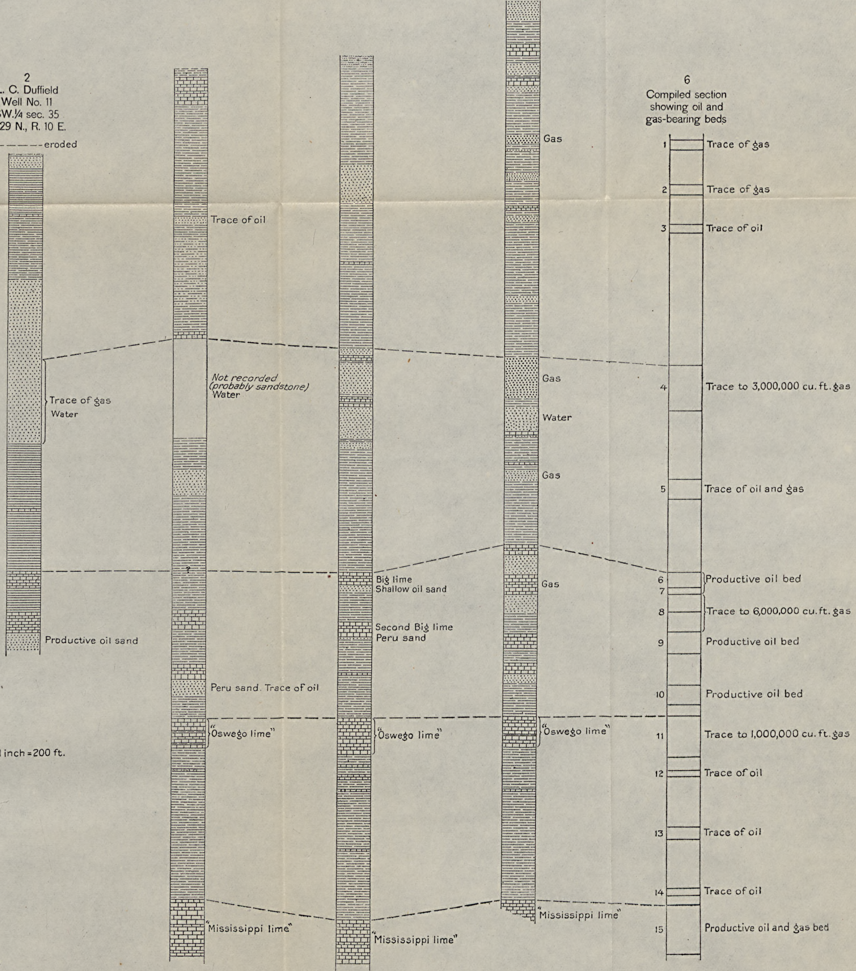
COMPARISON OF EXPOSED AND UNEXPOSED ROCKS AND STRATIGRAPHIC POSITIONS OF OIL AND GAS BEARING BEDS IN T. 28 N., RS. 9 AND 10 E., AND T. 29 N., R. 10 E.
