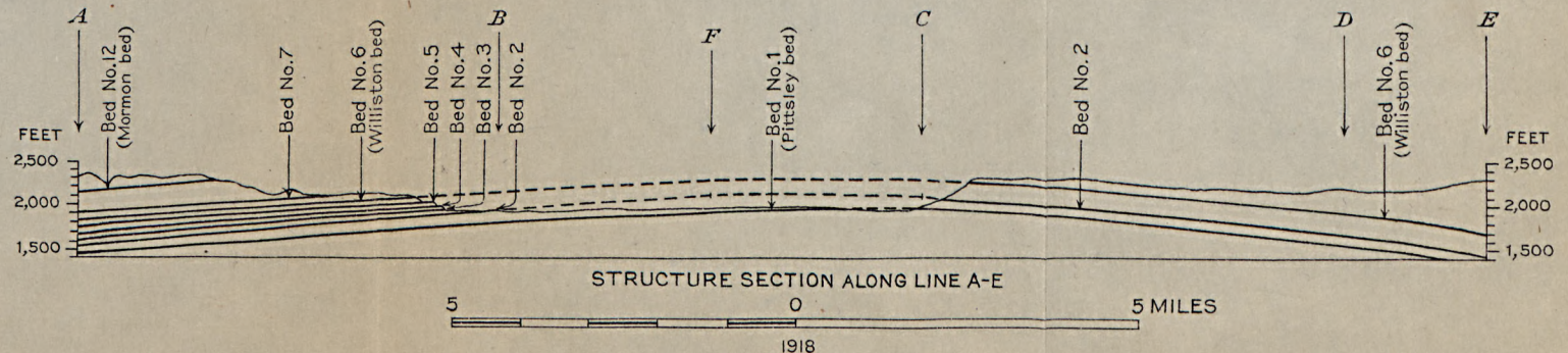
STRUCTURE MAP OF THE NESSON ANTICLINE, WILLIAMS COUNTY, N. DAK., AND SECTIONS SHOWING LIGNITE BEDS OF THE FORT UNION FORMATION EXPOSED NEAR THE ANTICLINE
