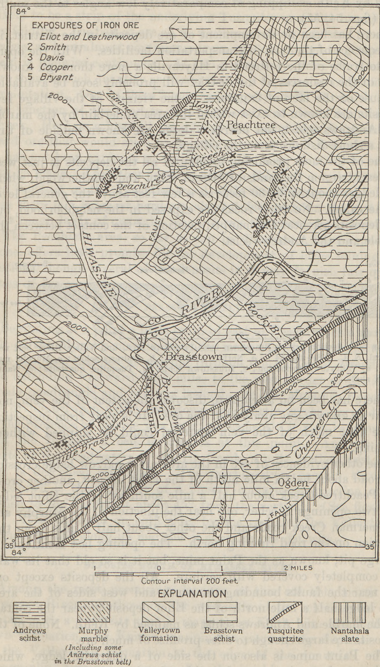
FIGURE 54.—Geologic map of the Peachtree area and the eastern part of the Brasstown belt, N. C. A-A', Line of right-hand portion of section, figure 55.
