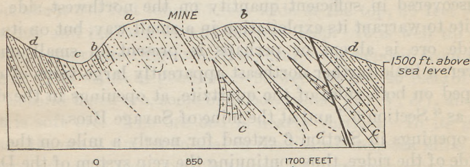
FIGURE 52.—Diagrammatic cross section through Fain-Hitchcock mine, near Murphy, N. C. a , Nottely quartzite; b , Andrews schist; c , Murphy marble; d , Valletown formation.
