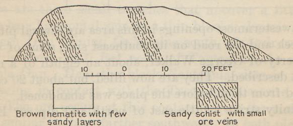
FIGURE 53.—Section across end of pit on J. W. Walker property, near Andrews, N. C.
