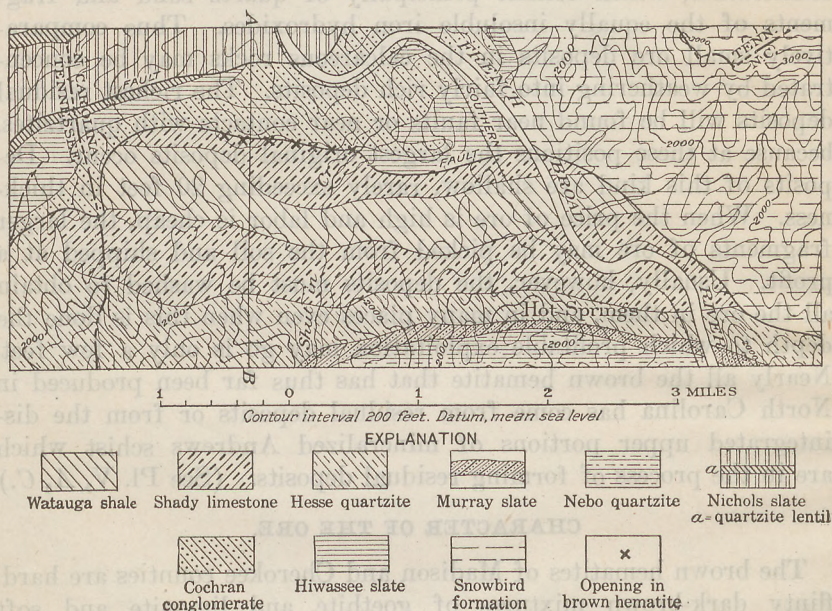
FIGURE 48.—Geologic map of area containing deposits of brown hematite at Tenneslina, near Hot Springs, N. C. A-B, Line of section, figure 49.
