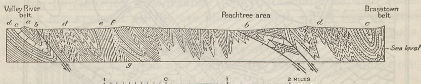
FIGURE 55.—Section across Brasstown belt, Peachtree area, and Valley River belt near Regal, N. C. (See fig. 54.) a , Nottely quartzite; b , Andrews schist; c , Murphy marble; d , Valletown formation; e , Brasstown schist; f , Tusquitee quartzite; g , Nantahala shale.
