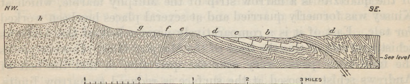
FIGURE 51.—Northwest-southeast section across Valley River hematite belt near Marble, N. C. b , Andrews schist; c , Murphy marble; d , Valletown formation; e , Brasstown schist; f , Tusquitee quartzite; g , Nantahala shale; h , Great Smoky formation.
