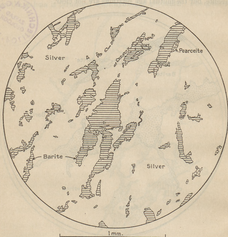
FIGURE 19.—Ragged replacement remnants of barite in native silver. Mollie Gibson mine, Aspen, Colo., from depth of about 500 feet. Camera lucida drawing from polished specimen.
