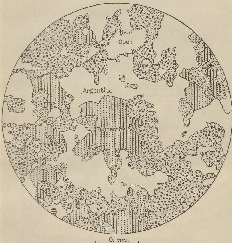
FIGURE 15.—Argentite, pearceite, and tennantite in irregular and apparently primary intergrowth. Aspen, Colo., precise location uncertain. Camera lucida drawing from polished specimen.
