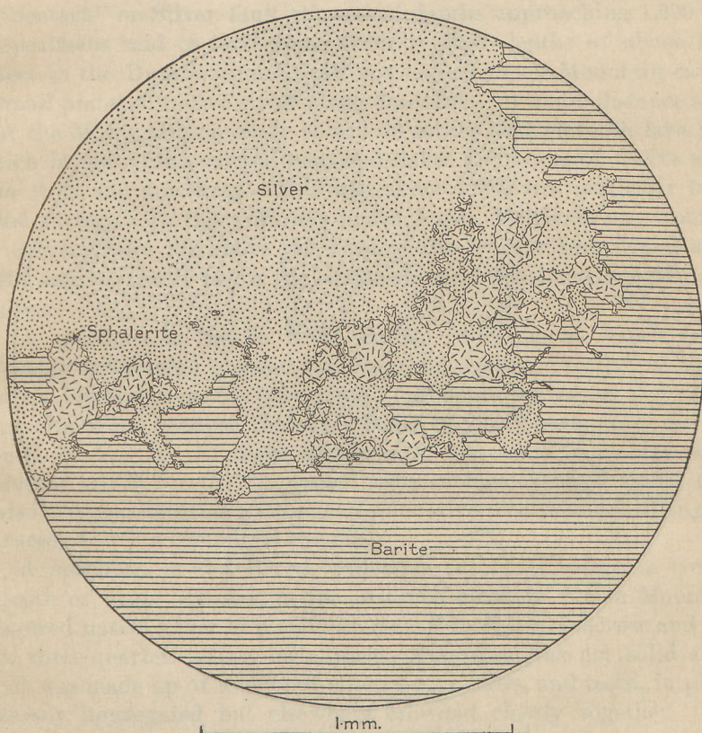
FIGURE 20.—Native silver replacing sphalerite and barite. Note exceedingly irregular silver boundaries and sphalerite replacement remnants within the silver. Small replacement remnants of tennantite (not shown) are scattered sparsely through the silver. Smuggler mine, Aspen, Colo., from depth of about 600 feet. Camera lucida drawing from polished specimen.
