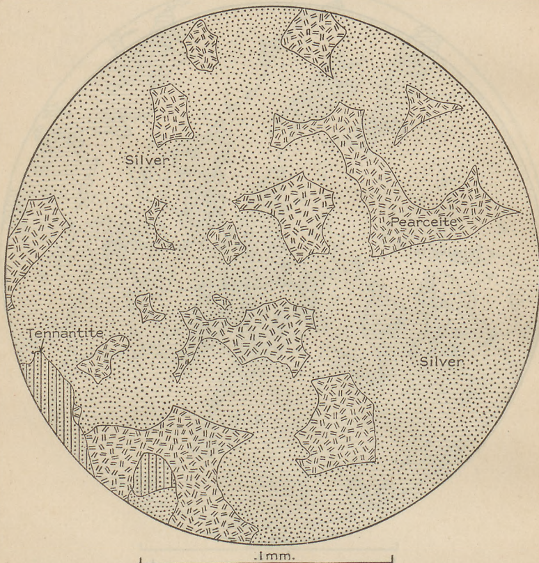
FIGURE 21.—Association of native silver and pearceite, Aspen, Colo. Note that the pearceite areas have curved outlines concave outward, suggesting that they are replacement remnants between areas of silver that have grown radially from numerous centers. Camera lucida drawing from polished specimen.
