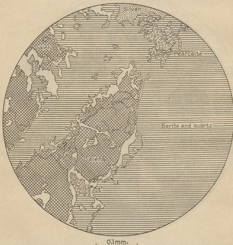
FIGURE 16.—Replacement of galena by a galena-like mineral, probably a lead-silver sulphide, followed by pearceite. The replacement follows the contacts between galena crystals or between galena and other minerals. Where replacement has proceeded further pearceite is developed, as at A and A'. Native silver occurs as a final replacement product in those parts of the specimen where pearceite is most abundant, as shown in the upper part of this figure. In parts of this specimen argentite is intimately associated with pearceite and seems to be of the same age. Mollie Gibson mine, Aspen, Colo. Camera lucida drawing from polished specimen.
