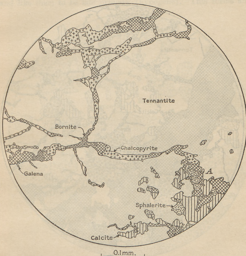
FIGURE 13.—Tennantite traversed by veinlets of chalcopyrite, galena, bornite, sphalerite, and calcite. These are in part replacement veinlets. Their transition, as at A, into irregular intergrowths with tennantite suggests that the veinlets are not much younger than the tennantite. Pearceite is a component of many similar veinlets in this specimen. All probably belong to a single period of primary mineralization. Smuggler Hill workings, block 30, Aspen, Colo., thirteenth level. Camera lucida drawing from polished specimen.
