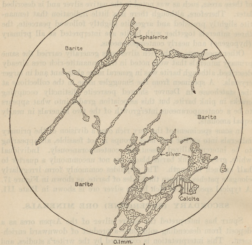
FIGURE 17.—Replacement of sphalerite stringers in barite by native silver. Smuggler mine, Aspen, Colo., from depth of 140 feet in shaft. Camera lucida drawing from polished specimen.
