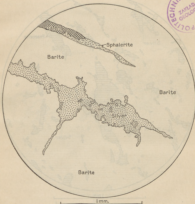
FIGURE 18.—Replacement of barite by native silver. Smuggler mine, Aspen, Colo., from depth of 140 feet in shaft. Process began with replacement of narrow areas of sphalerite between bladelike crystals of sphalerite and spread to the bordering barite. Camera lucida drawing from polished specimen.
