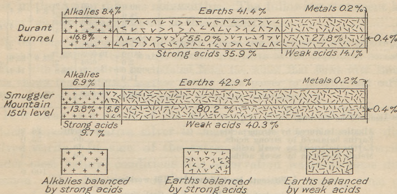
FIGURE 22.—Composition diagrams of cool descending mine waters of Aspen, Colo.
