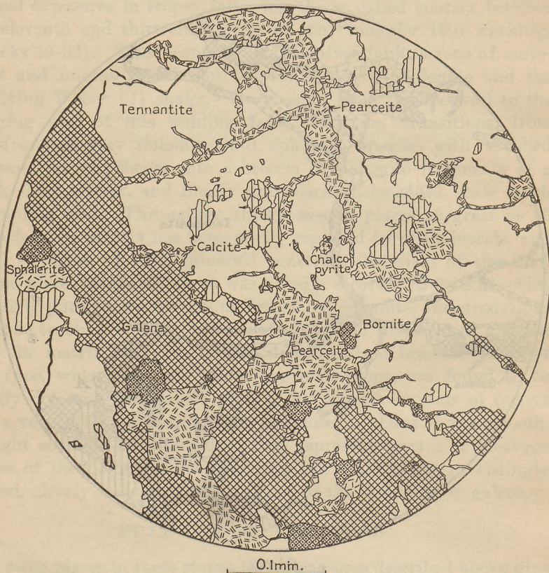
FIGURE 14.—Tennantite traversed by late primary replacement veinlets of pearceite, base-metal sulphides, and calcite. The textural relations suggest that some calcite and base-metal sulphides crystallized contemporaneously with the tennantite, but where they form veinlets they are clearly slightly younger. Smuggler Hill workings, block 30, Aspen, Colo., thirteenth level. Camera lucida drawing from polished specimen.
